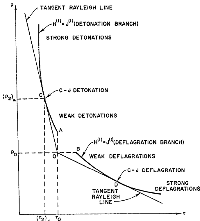
FIG 2 Hugoniot curve H^{(1)} = J^{(1)} of reaction products, with sections corresponding to strong, Chapman-Jouquet, and weak detonations and deflagrations
